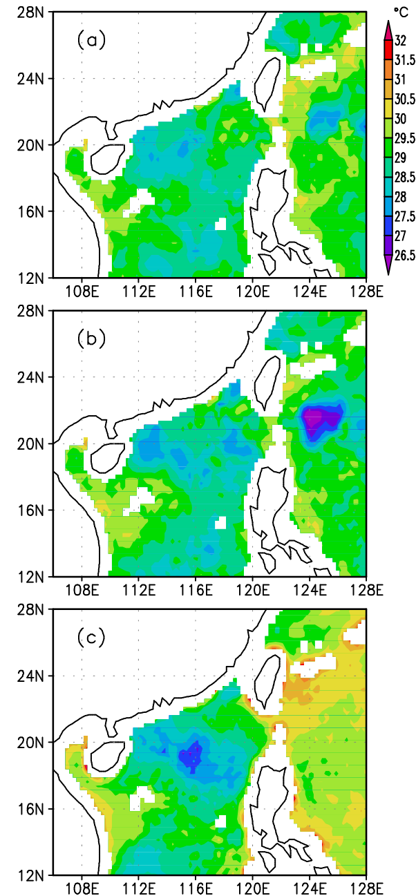
Fig.1 The distribution of TMI-AMSRE SST, (a) daily averaged SST on September 1, 2003, (b) daily averaged SST on September 2, 2003, and (c) weekly averaged SST.
